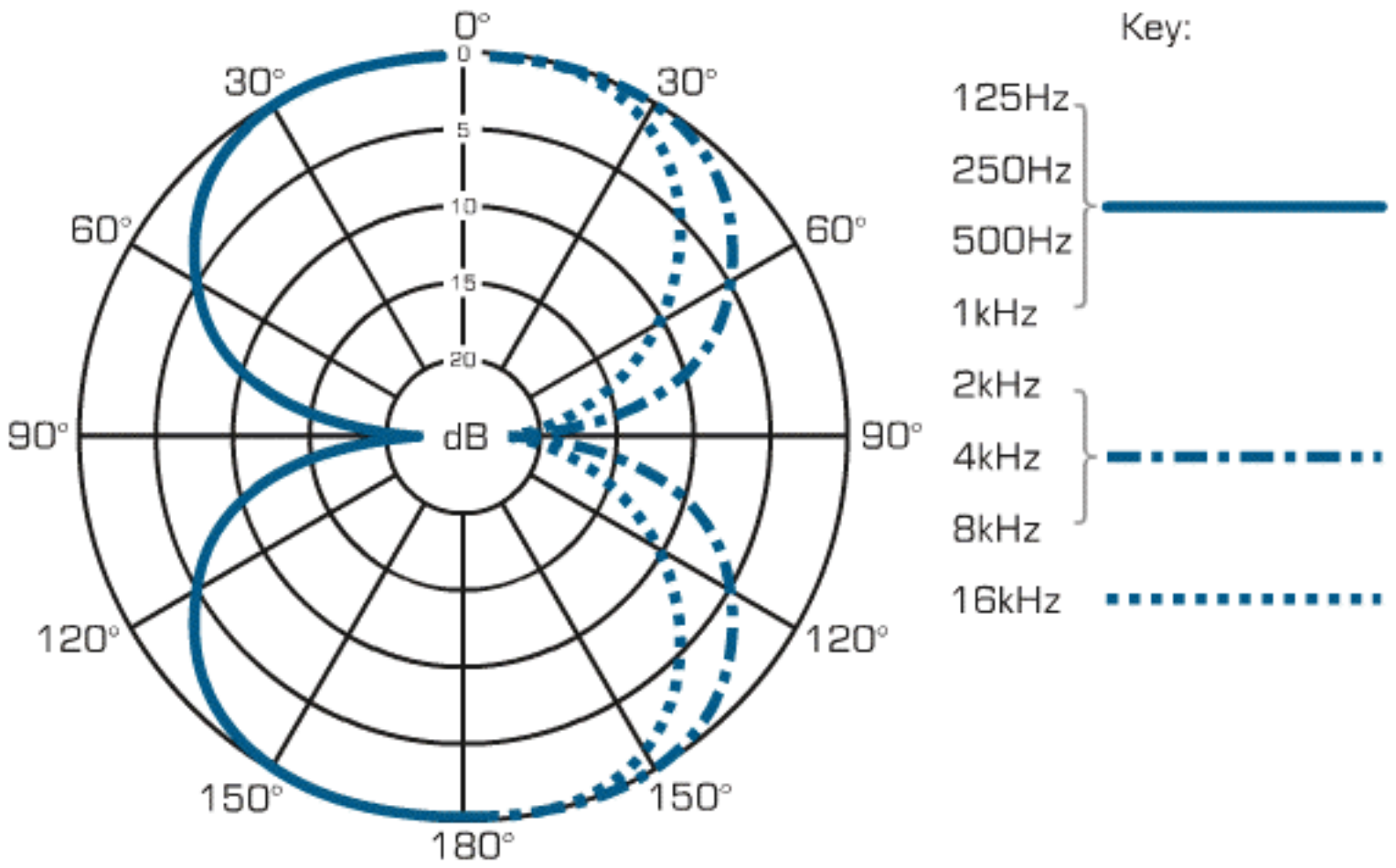
Polar curve: Figure of 8
