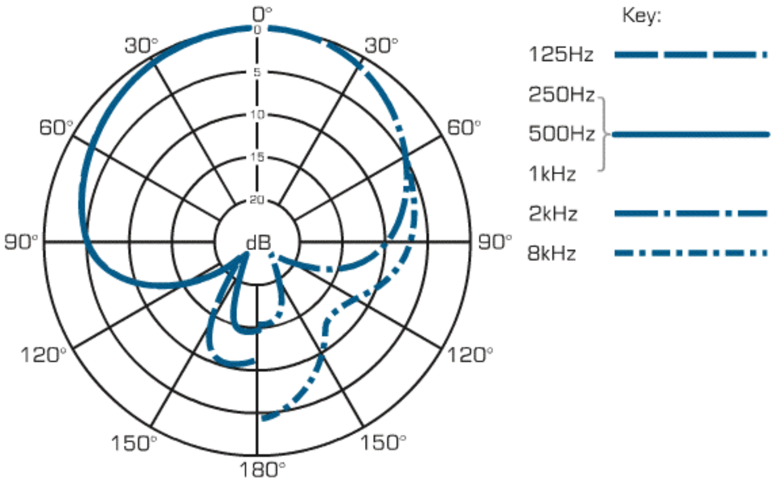
Polar curve: Hypercardioid
