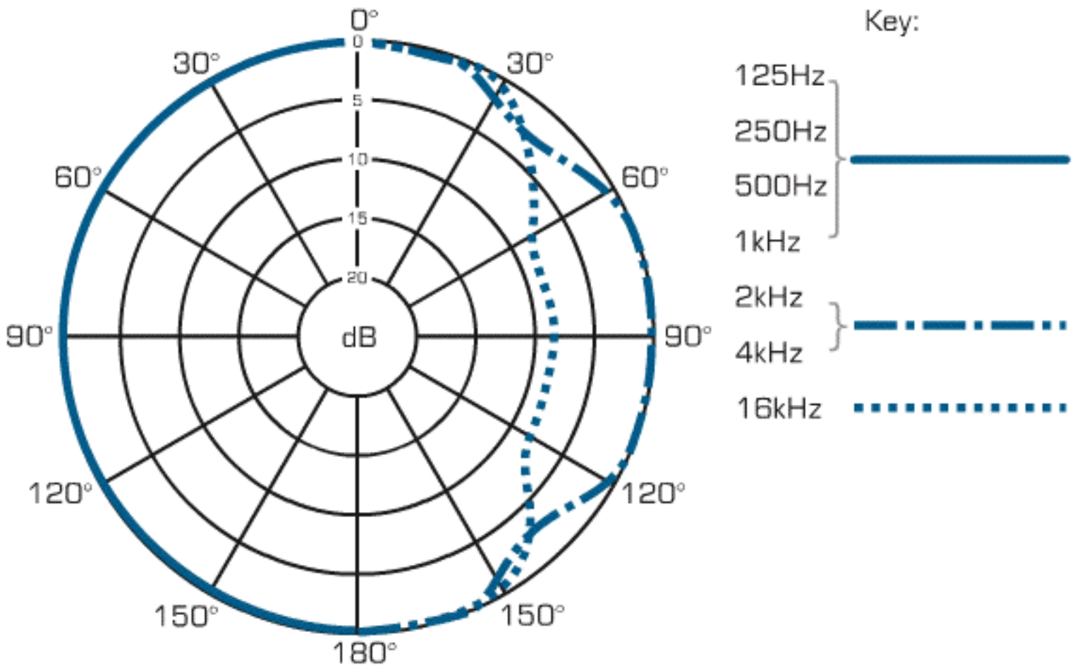
Polar curve: Omni
